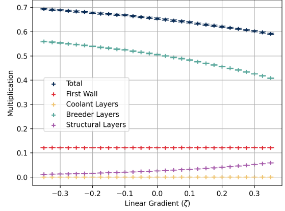
(b) Neutron multiplication contribution
